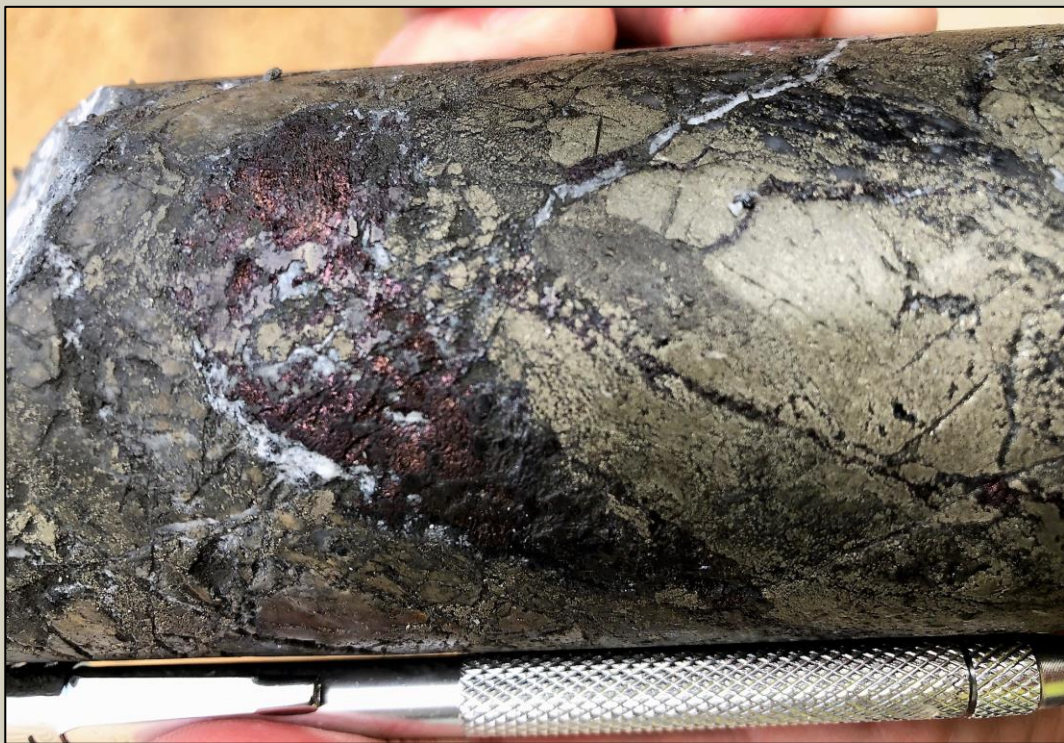
Photo 1. Bornite-chalcocite-pyrite mineralisation at 926.9m in SMD044.
