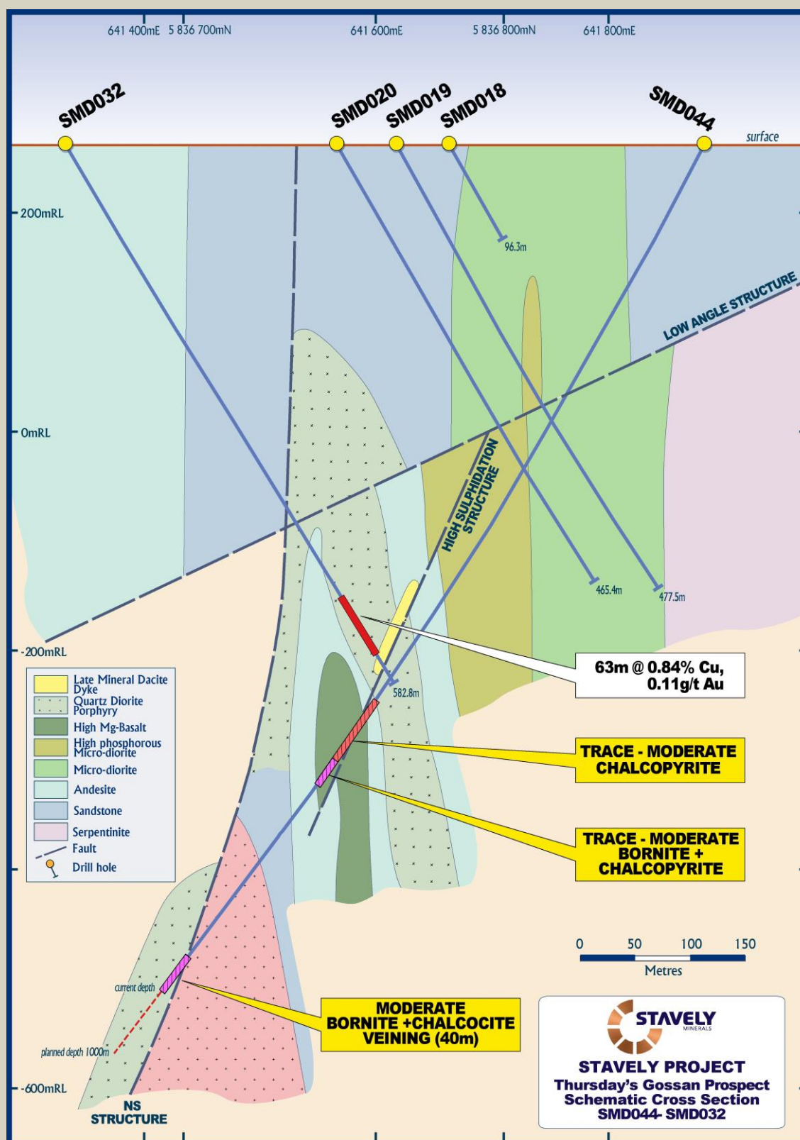
Figure 3. SMD044 section.
